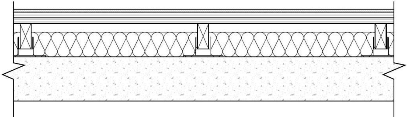
Figure 2 Cross section of A1-019524-03F.
